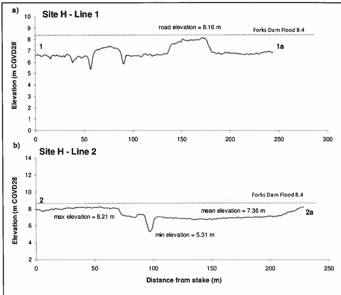
Figure 29: Cross sectional profiles at Site H on the western shore of Pisiquid Lake. Location of profiles indicated on Figure 28.
